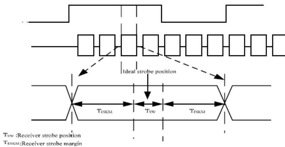
LVDS timing(3)
