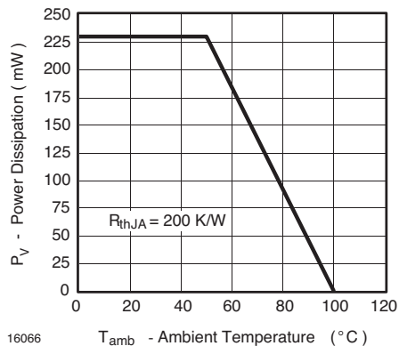
Figure 3. Power Dissipation vs. Ambient Temperature for InGaN
