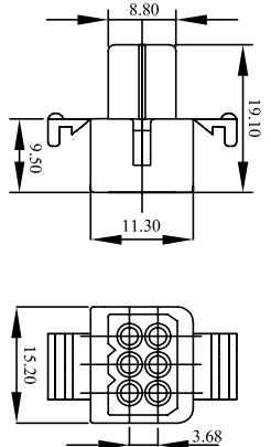
WW158B-F06E(5A/250V)
