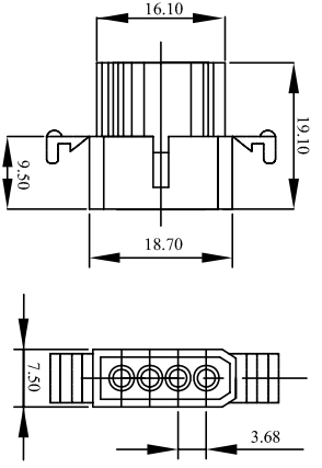
WW158B-F04E(5A/250V)
