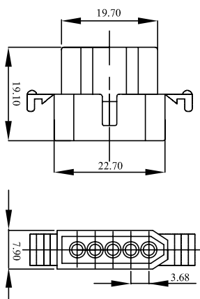
WW158B-F05E(5A/250V)
