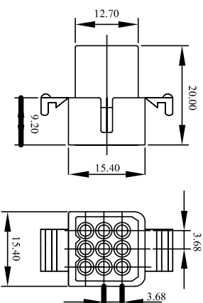
WW158B-F09E(5A/250V)
