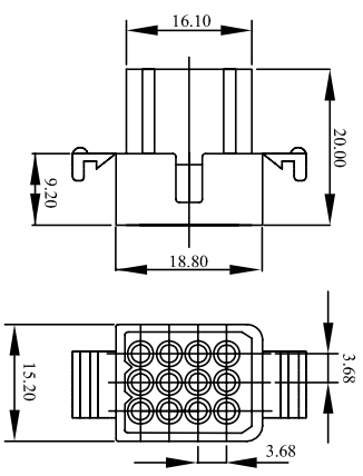
WW158B-F12-1E(5A/250V)
