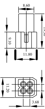
WW158B-F04-1E(10A/250V)
