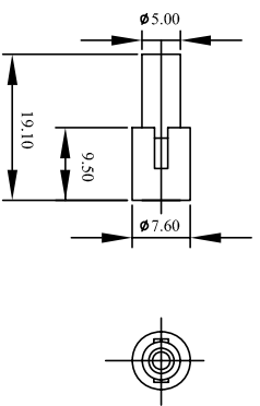
WW158B-F01(5A/250V)
