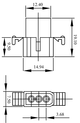
WW158B-F03E(5A/250V)
