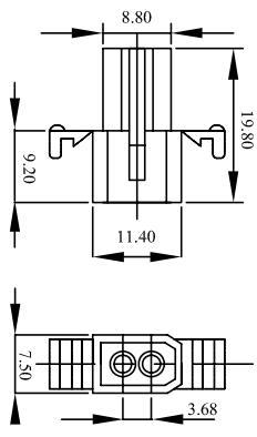
WW158B-F02E(5A/250V)
